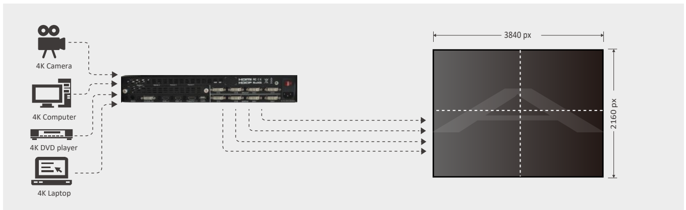
Application 4: display different image on 4 LED screens
